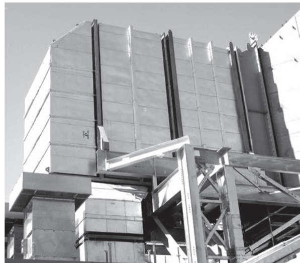
COMBINED CYCLE POWER PLANT INTAKE SILENCING
